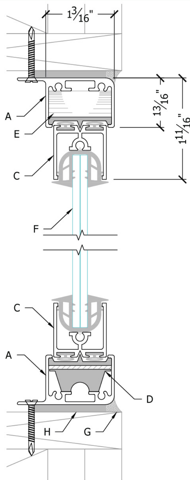
A SILL AND HEADER DETAIL
