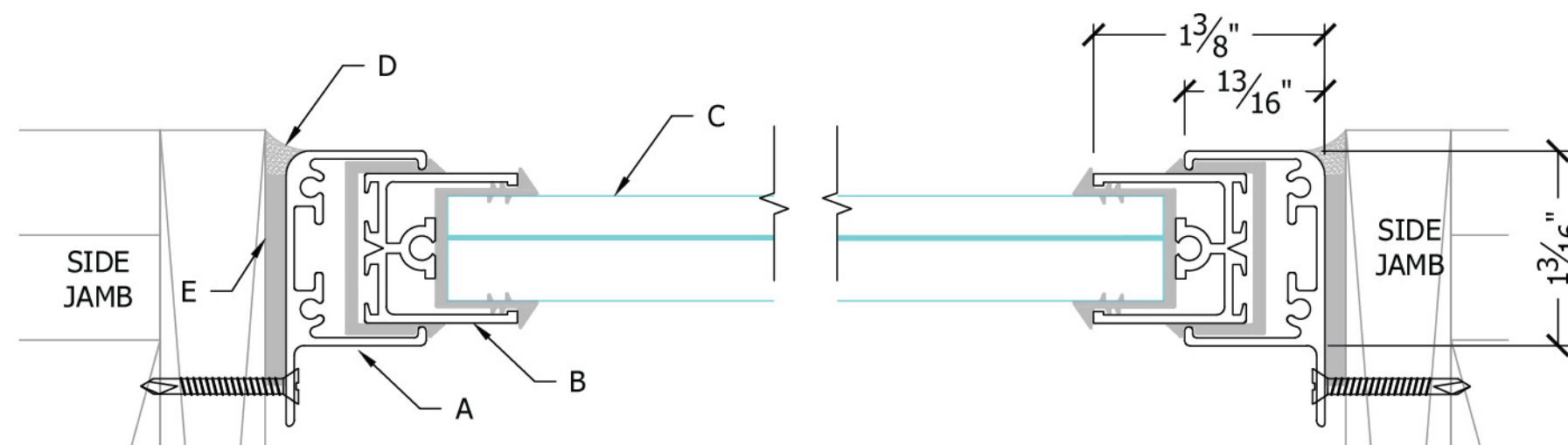
B SIDE WALL DETAIL SCALE: 1:1
